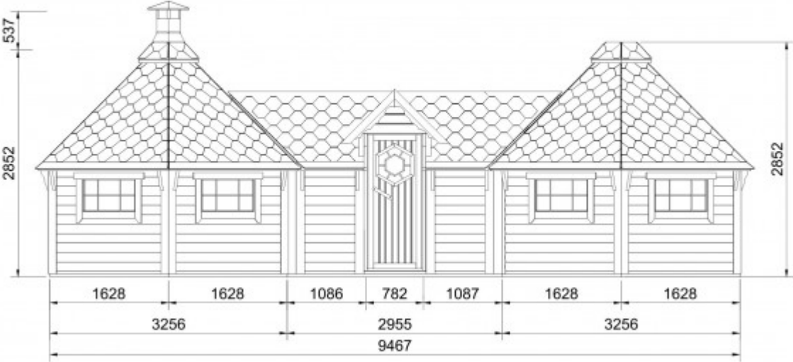
Front view
